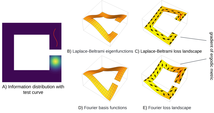
Fig. 3. Effect of modifying the ergodic metric to use the Laplace-Beltrami eigenfunctions. (A) A C-shaped map with an information peak (yellow) and test curve (red) are separated by a gap. Both basis function choices depend only on the geometry of the obstacle map and can be compared in figures B and D. The Laplace-Beltrami eigenfunctions (B) have the correct sense of continuity influenced by the boundaries of the free space, while the ordinary Fourier basis functions (D) try to maintain continuity within the gap. As a result, the Laplace-Beltrami loss landscape (C) smoothly pushes the test curve around the central obstacle, while the Fourier loss landscape (E) gets trapped in a local minima.
