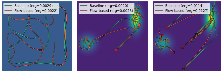
Fig. 5. Results for obstacle-free square map comparing our and the baseline methods. From left to right, we have the trajectories generated for the uniform, nonuniform, and multi-agent nonuniform test cases. The ergodic metric value for each trajectory is shown in the figure legend.
