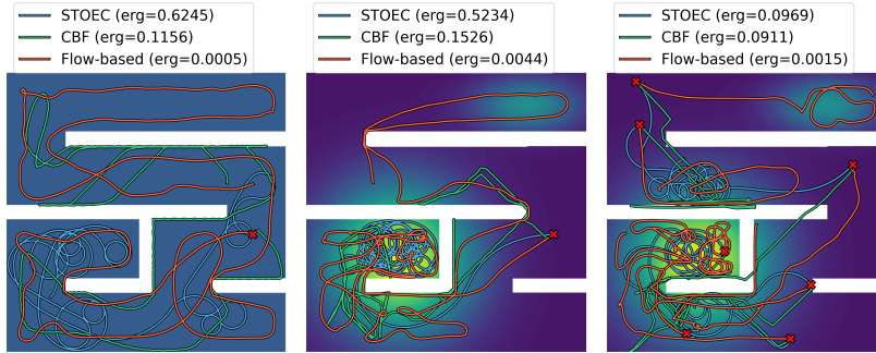
Fig. 6. Results for maze map comparing our and prior methods. From left to right, we have the trajectories generated for the uniform, nonuniform, and multi-agent nonuniform test cases. The ergodic metric value for each trajectory is shown in the figure legend, calculated using the Laplace-Beltrami ergodic metric.
