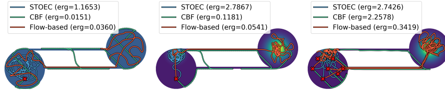
Fig. 7. Results for the rooms map comparing our and prior approaches. From left to right, we have the trajectories generated for the uniform, nonuniform, and multi-agent nonuniform test cases. The ergodic metric value for each trajectory is shown in the figure legend, calculated using the Laplace-Beltrami ergodic metric.
