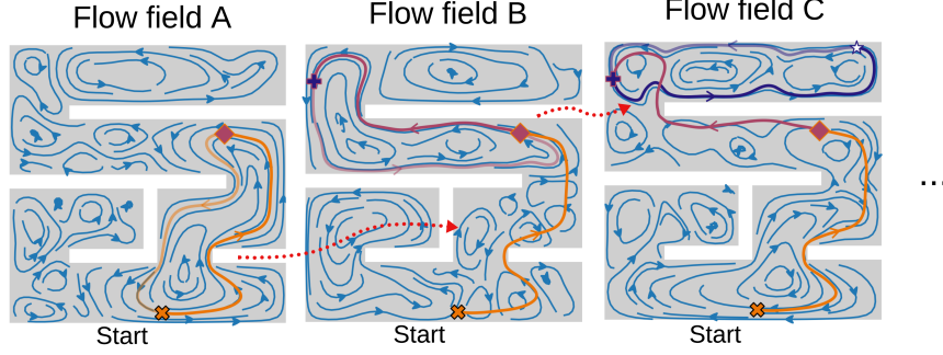
Fig. 2. Example measure-preserving flows for a uniform information distribution on a maze-like space, drawn in blue. (A) Starting from an initial condition marked by the brown X, the brown line represents a trajectory traced by following the flow field lines. Note that the flow lines form stationary limit cycles, as shown by the faded brown extension, so the robot will simply trace the same cycle repeatedly. (B) By cleverly switching the underlying flow field when the robot reaches the magenta diamond, we can escape the limit cycle and cover more space. (C) We can repeat this process when the robot reaches the purple plus, extending the trajectory to cover more of the map. This process can be repeated again when the robot reaches the white star ad infinitum.
